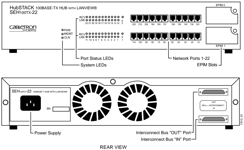
Figure 2-1 Front and Rear Views of the SEH100TX-22
